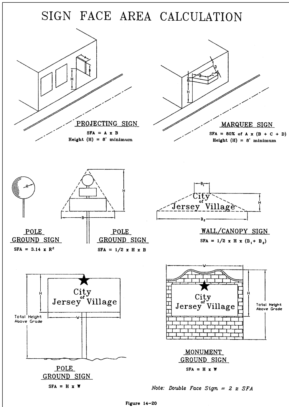
Figure 14-20 Sign Face Area Calculation
